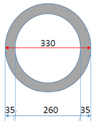
Retort tube cross section
