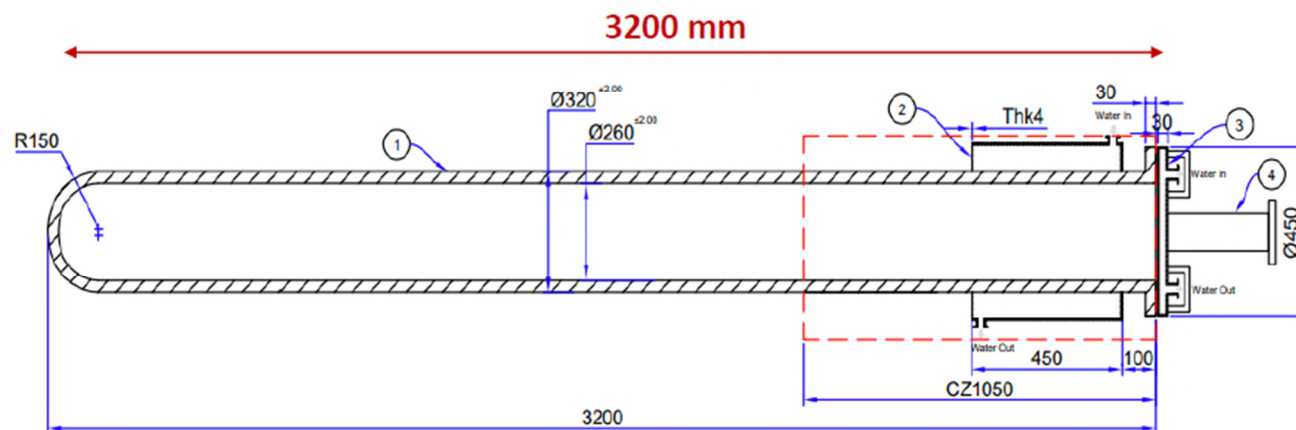
Sectional Front view A-A'
