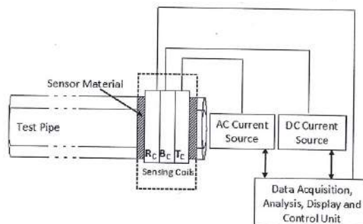
Fig-1. Scheme of the Magnetostrictive Sensing Device.
