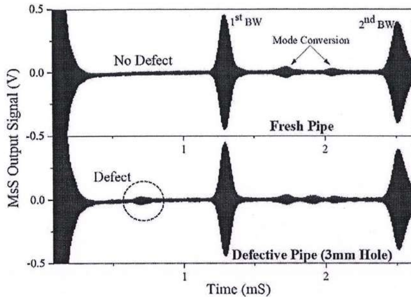
Fig-2. Magnetostrictive sensor signal from a pipe
